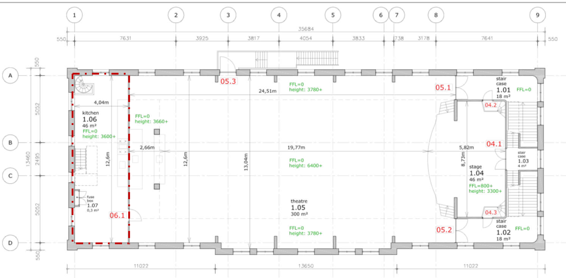
first floor
